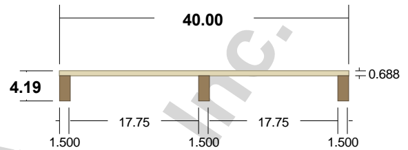
End View
